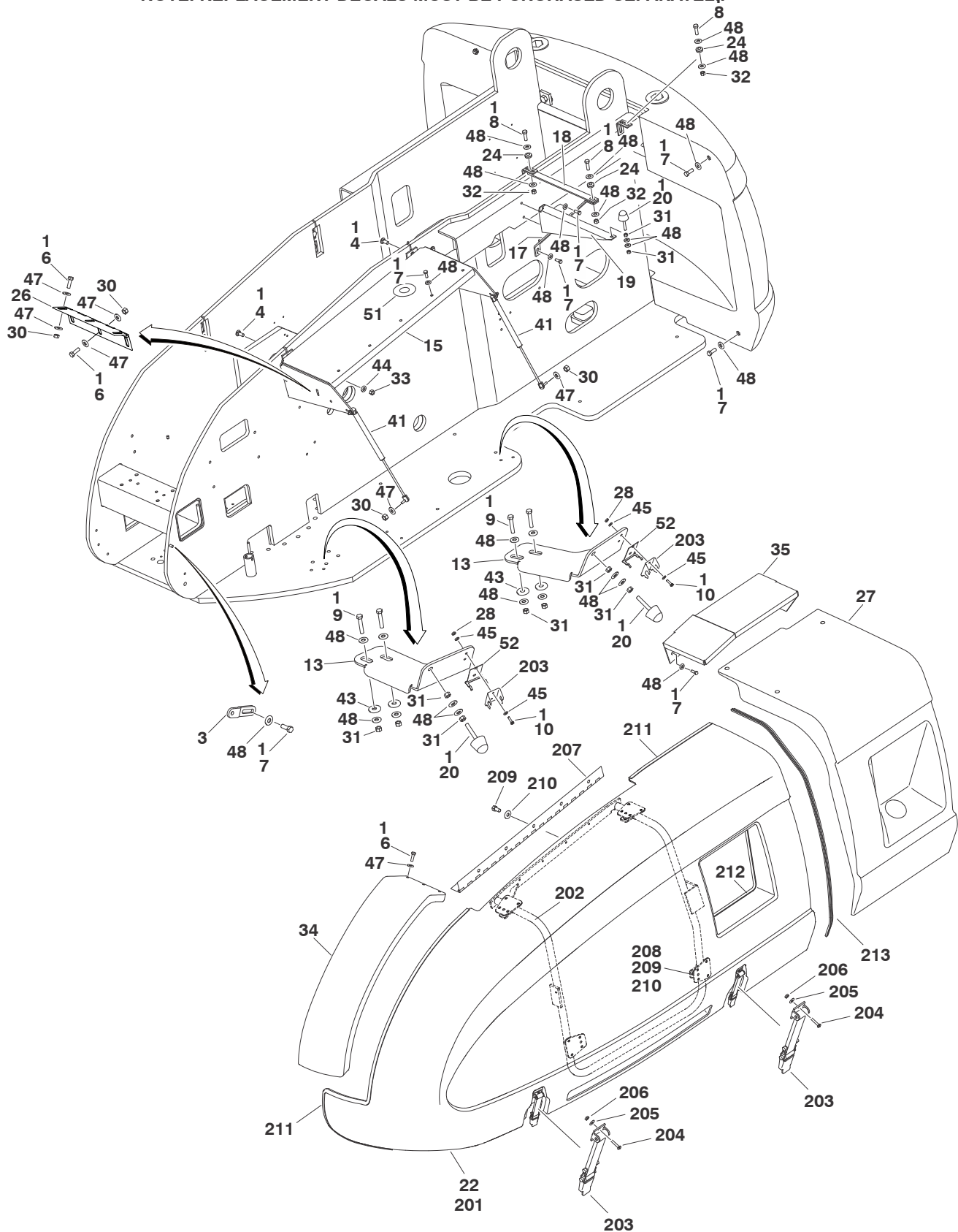
FIGURE 2-16. HOODS INSTALLATION (ABS)
