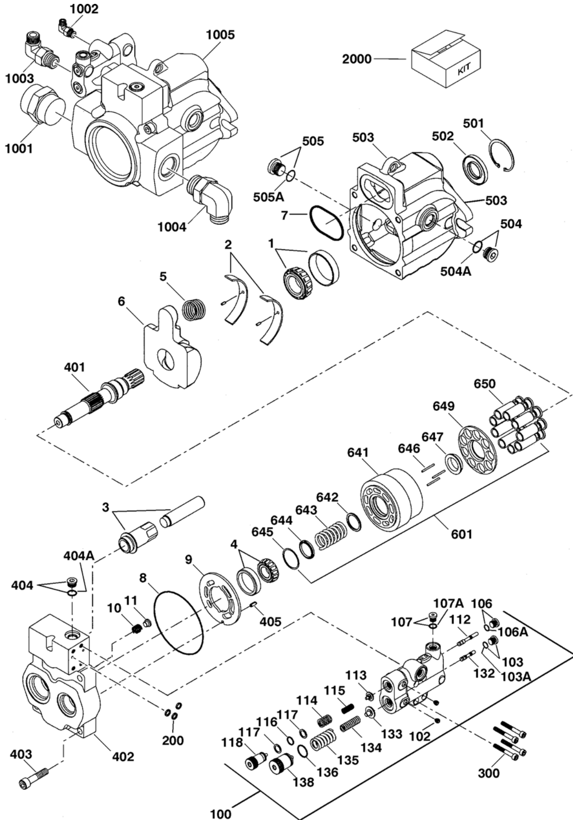
FIGURE 2-10. LOAD SENSING PUMP ASSEMBLY
