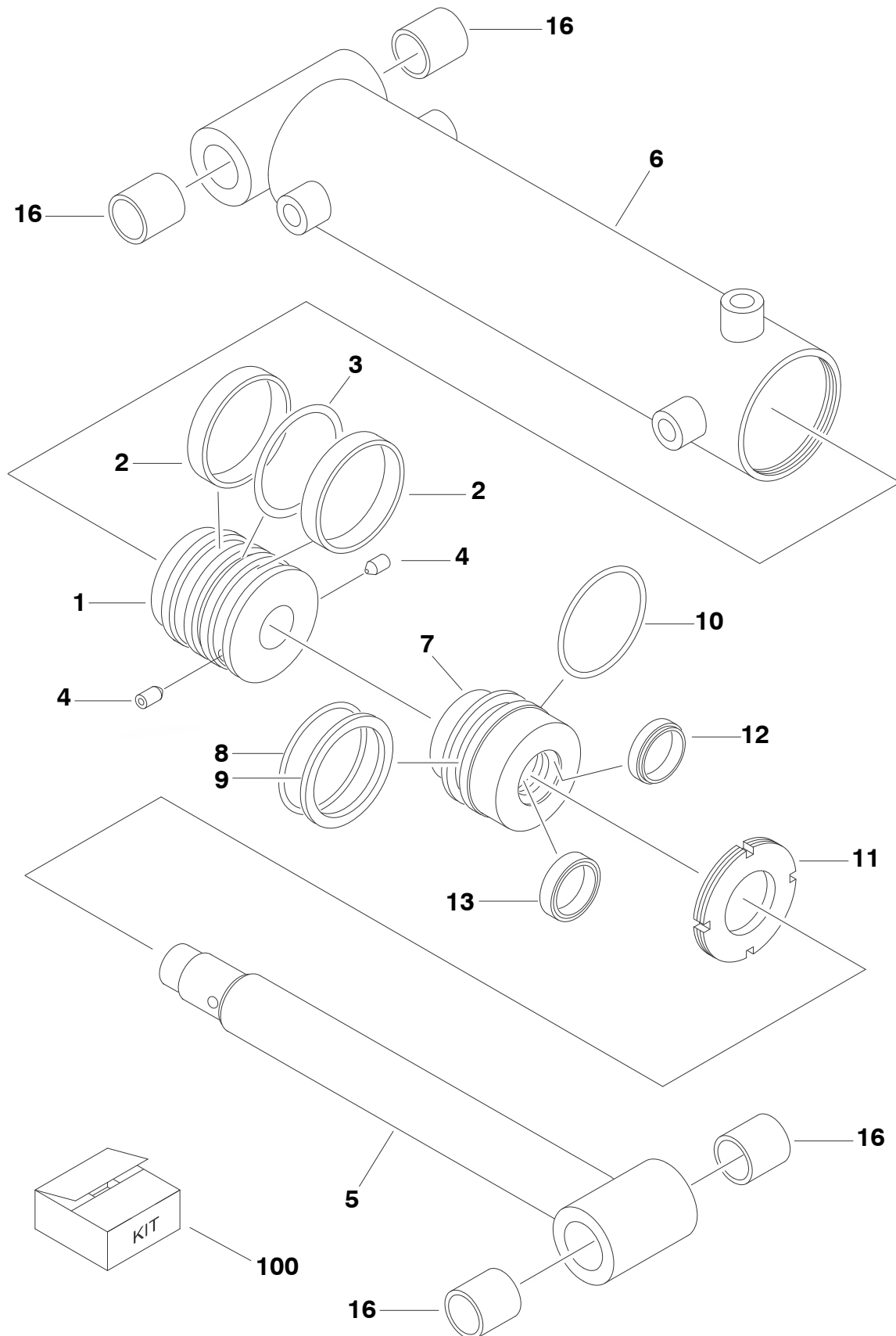
FIGURE 5-6. STEER CYLINDER ASSEMBLY (USA BUILT MACHINES SN 03000142666 TO SN 0300182743 ONLY & CHINA BUILT MACHINES SN B300000100 TO PRESENT ONLY)
