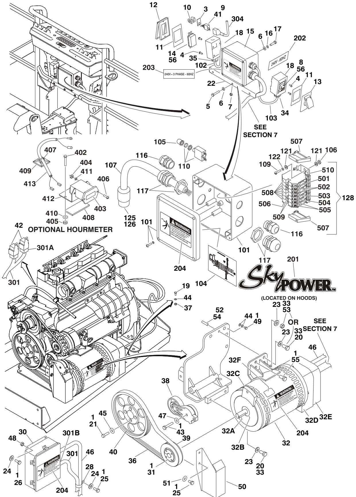
FIGURE 2-22. 7500W SKYPOWER GENERATOR INSTALLATION - CATERPILLAR & DEUTZ ENGINES
