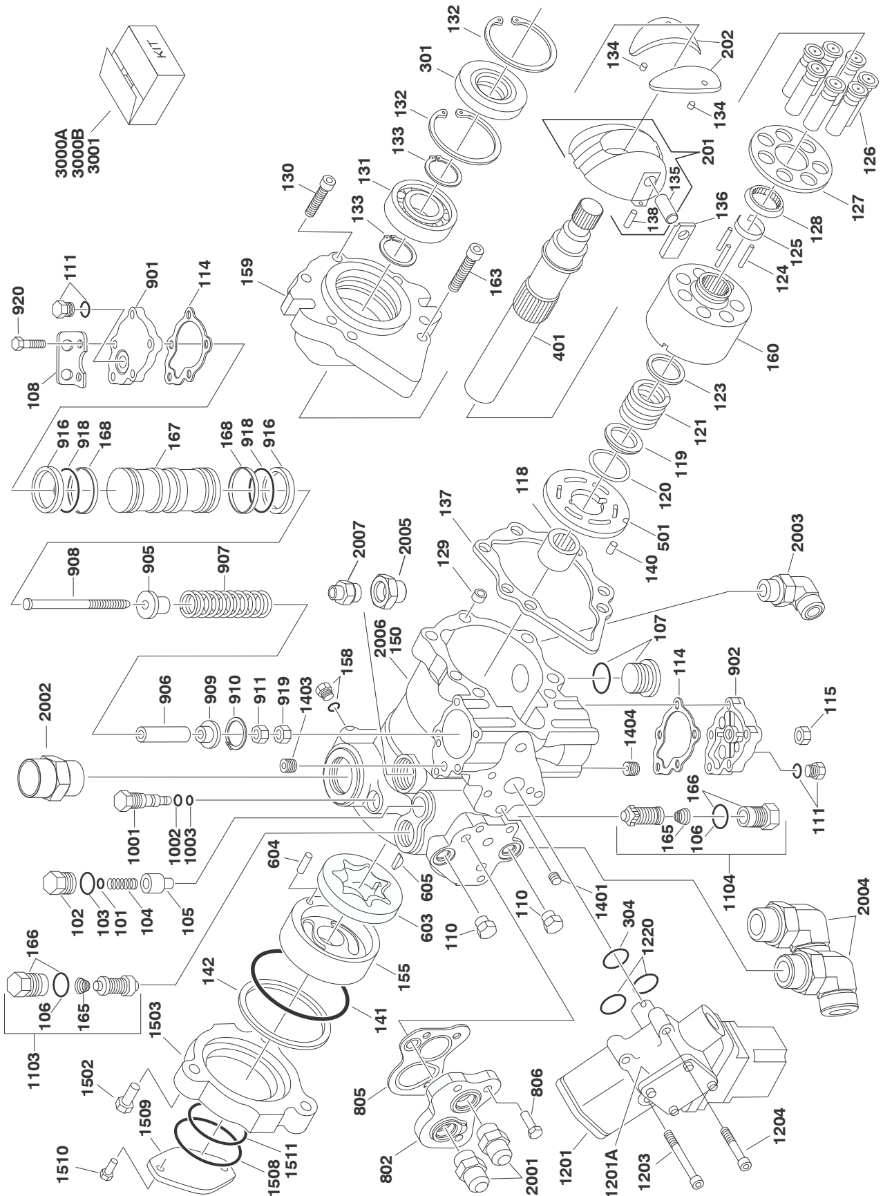
FIGURE 2-8. PUMP ASSEMBLY (SAUER-DANFOSS)
