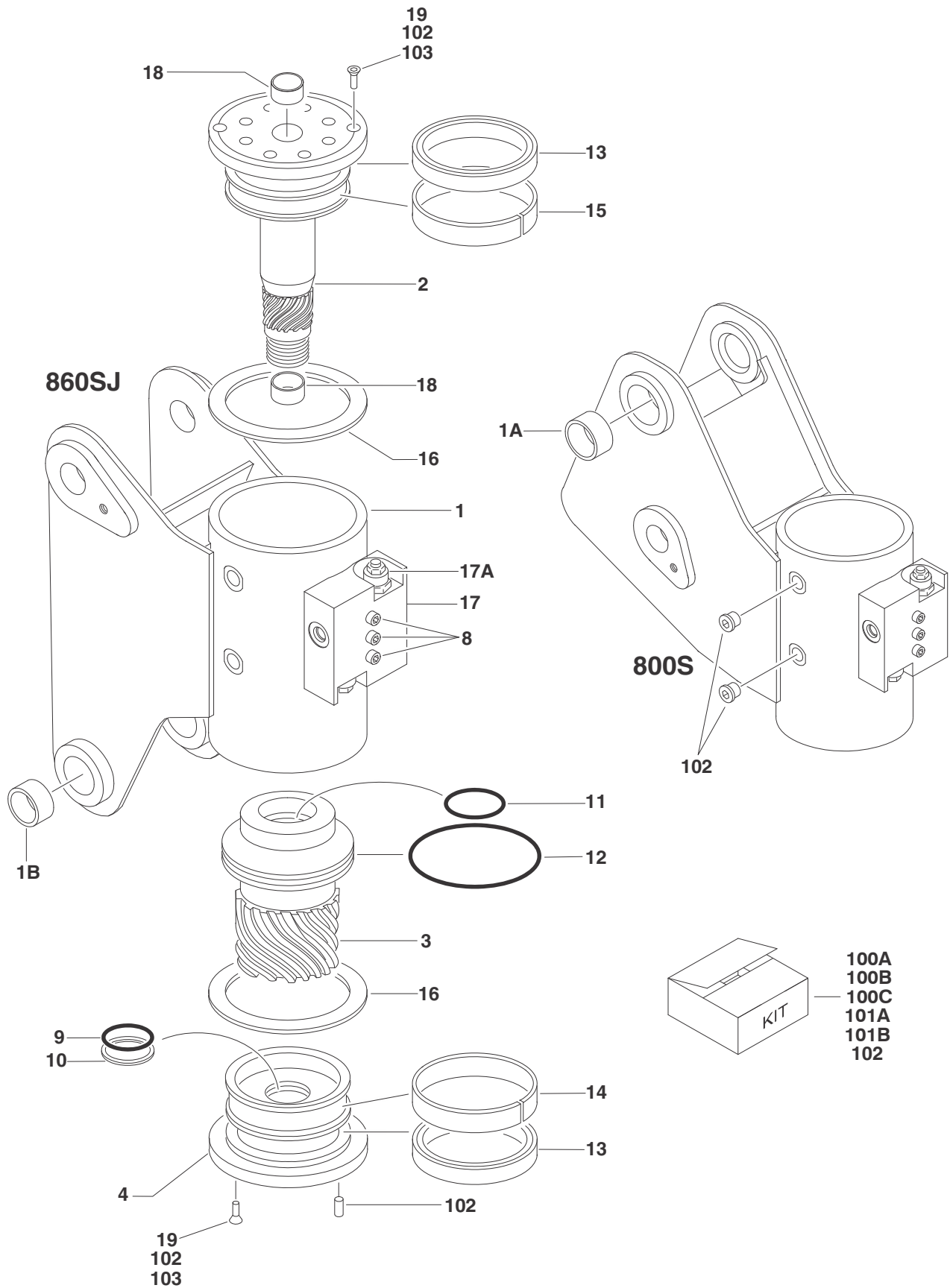
FIGURE 3-5. ROTATOR ASSEMBLIES
