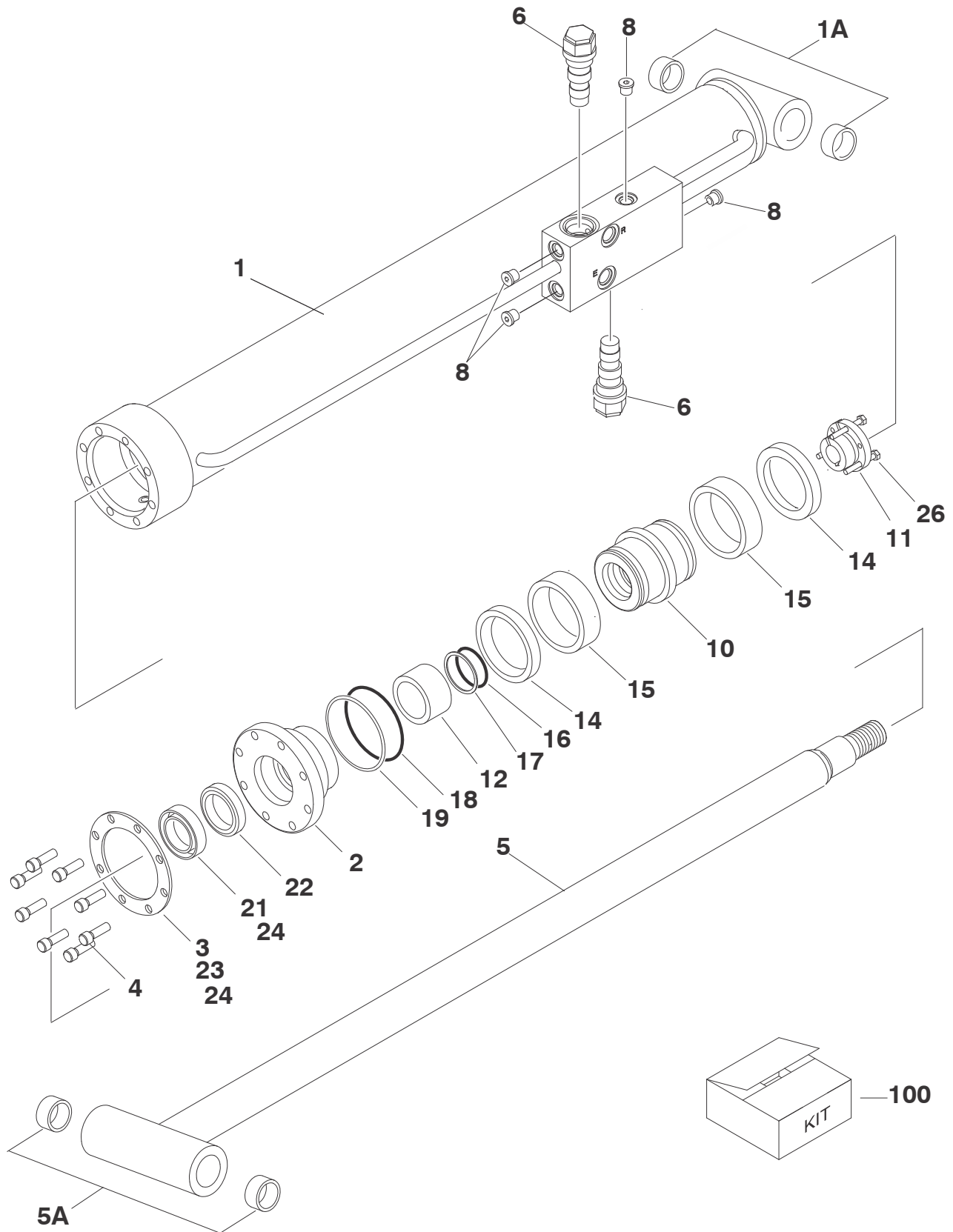
FIGURE 5-2. LIFT CYLINDER ASSEMBLY - JIB (860SJ ONLY)
