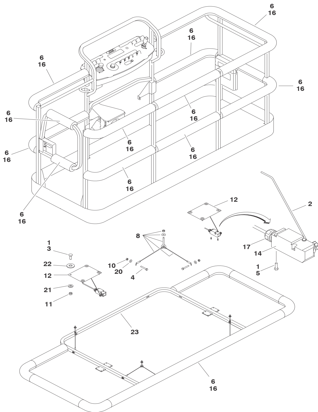
FIGURE 4-6. SOFT TOUCH SYSTEM INSTALLATION (OPTIONAL)
