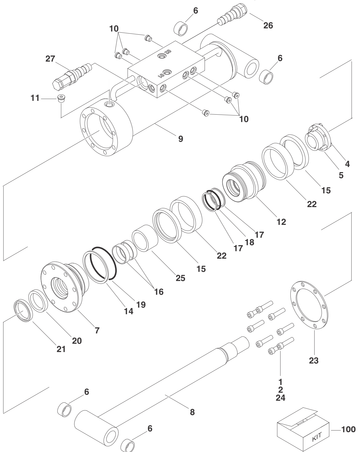
FIGURE 5-4. PLATFORM LEVEL CYLINDER ASSEMBLY
