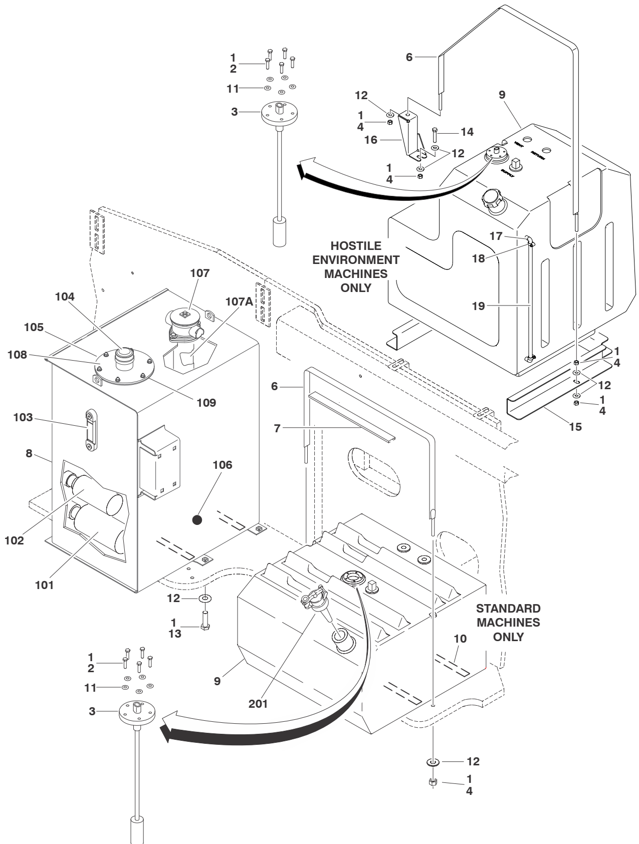
FIGURE 2-11. TANK INSTALLATIONS
