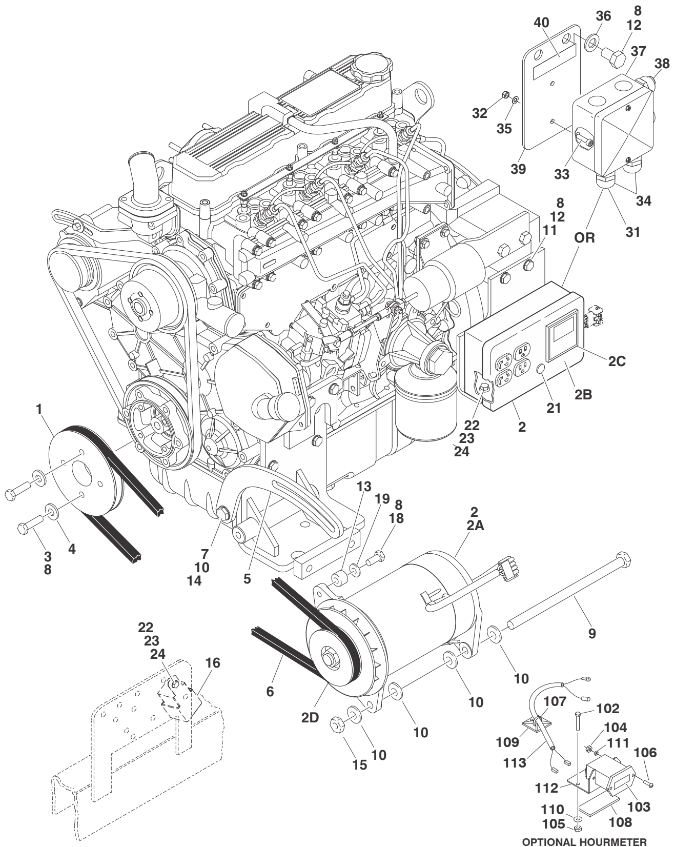
FIGURE 2-19. 2500W GENERATOR INSTALLATION - CATERPILLAR MACHINES (OPTIONAL)
