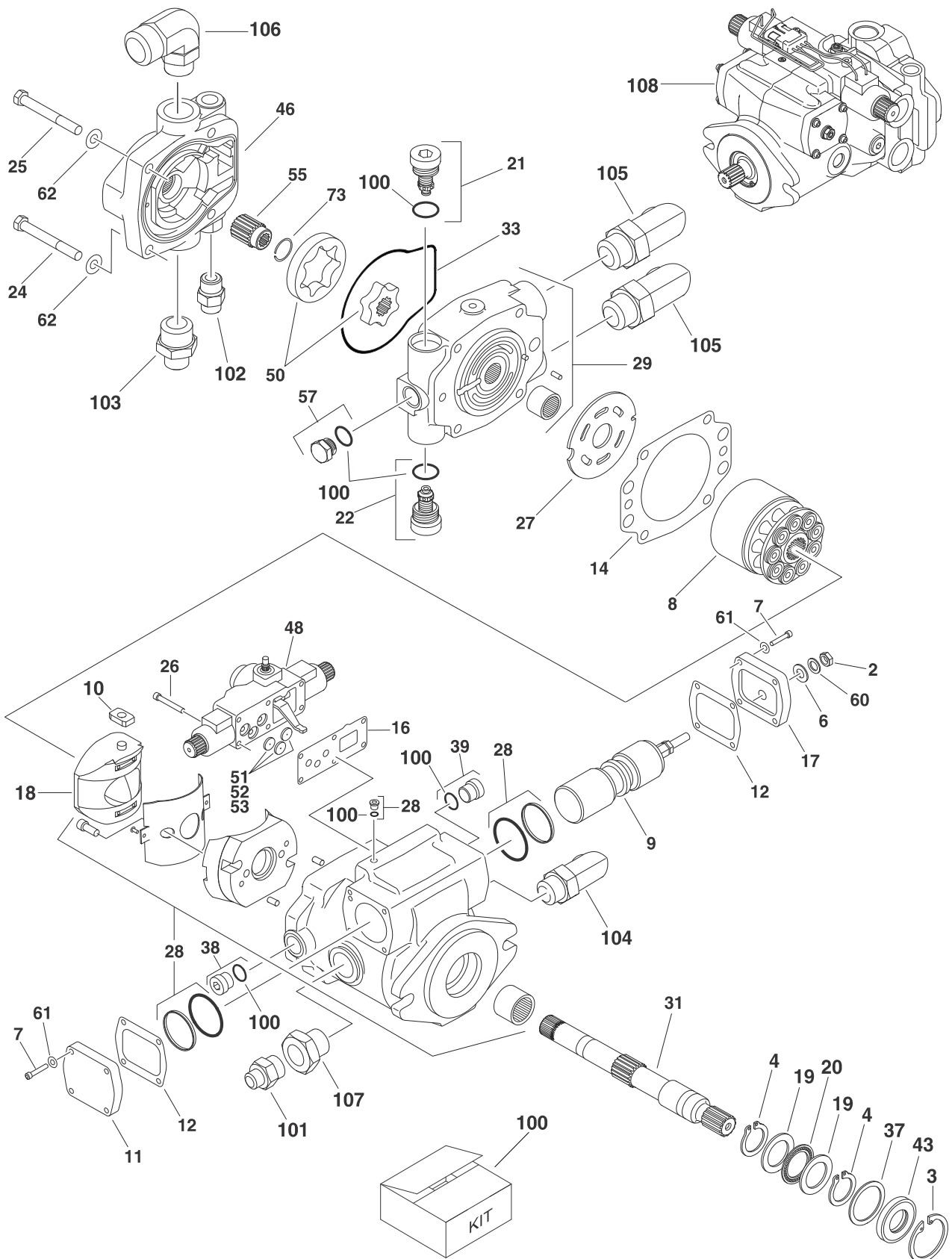
FIGURE 2-9. PUMP ASSEMBLY (EATON)
