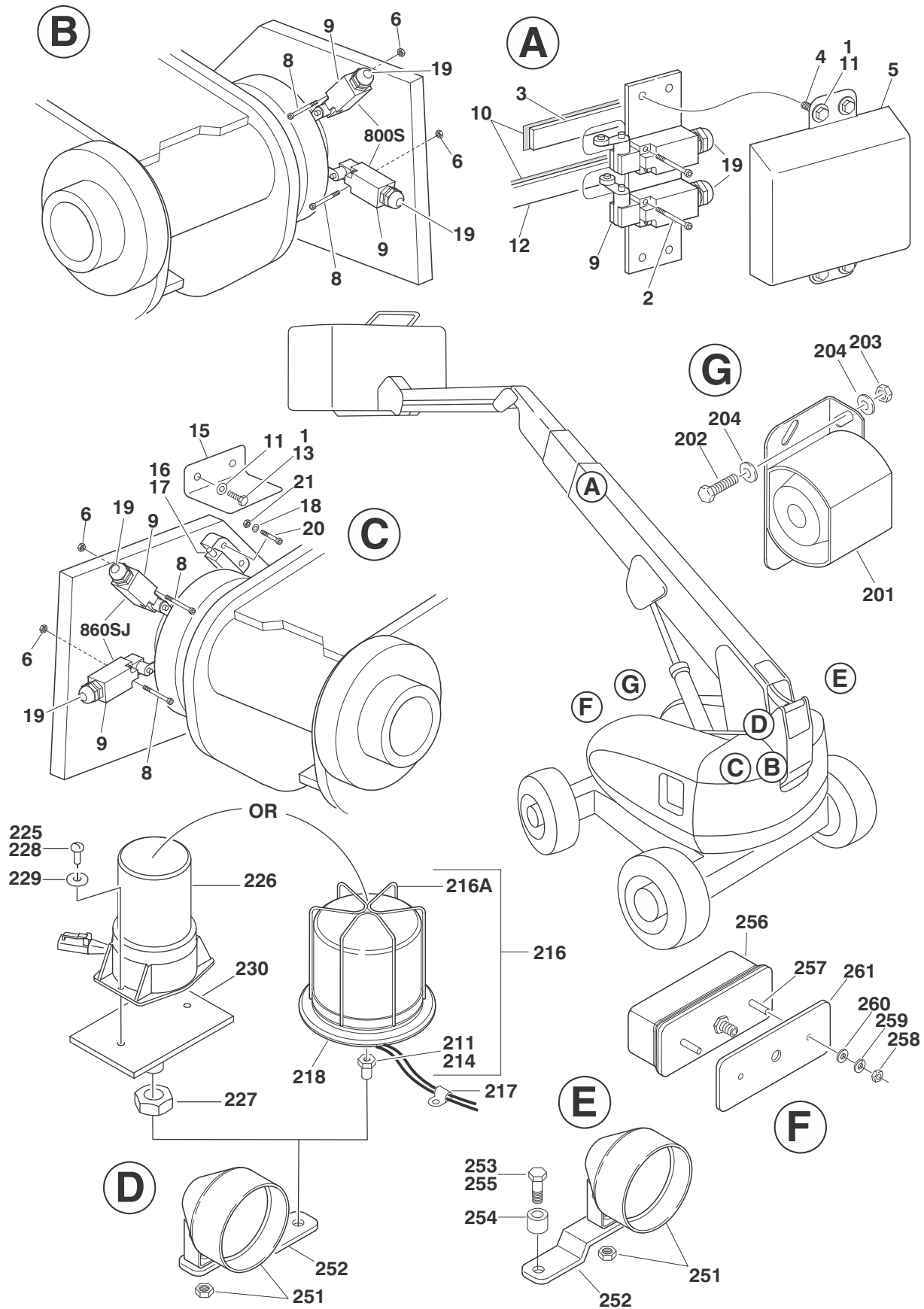
FIGURE 2-15. LIMIT SWITCHES, LIGHTS & ALARM INSTALLATIONS
