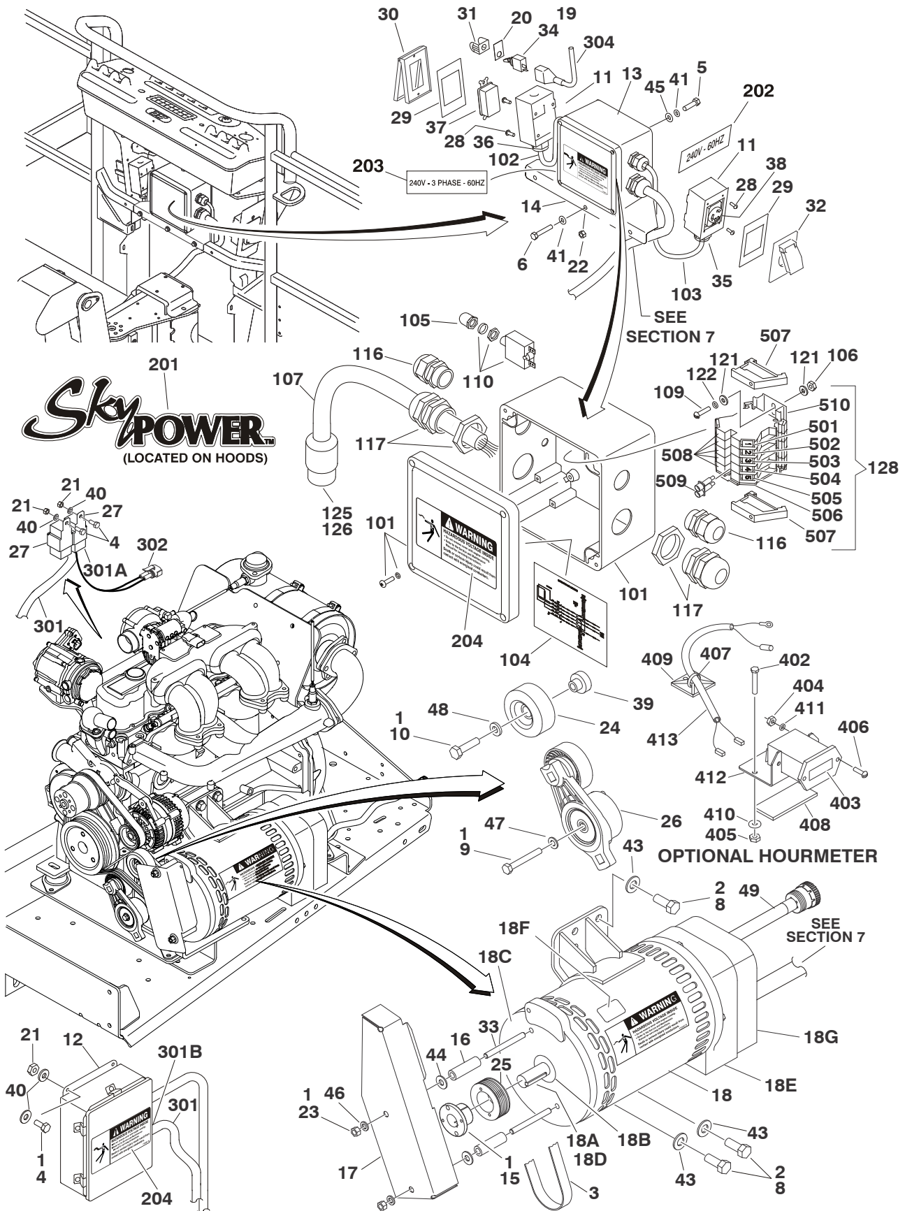
FIGURE 2-23. 7500W SKYPOWER GENERATOR INSTALLATION - GM ENGINES
