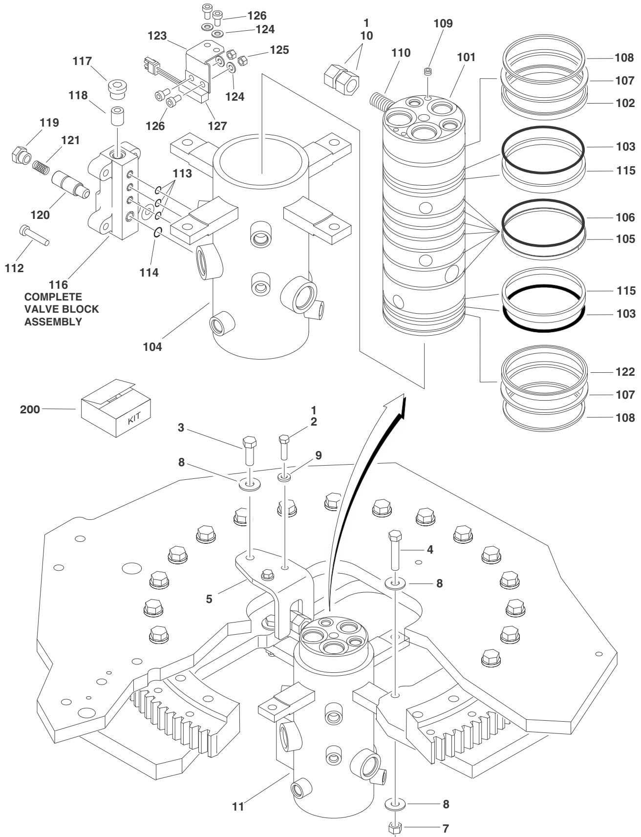
FIGURE 2-13. ROTARY COUPLING INSTALLATION
